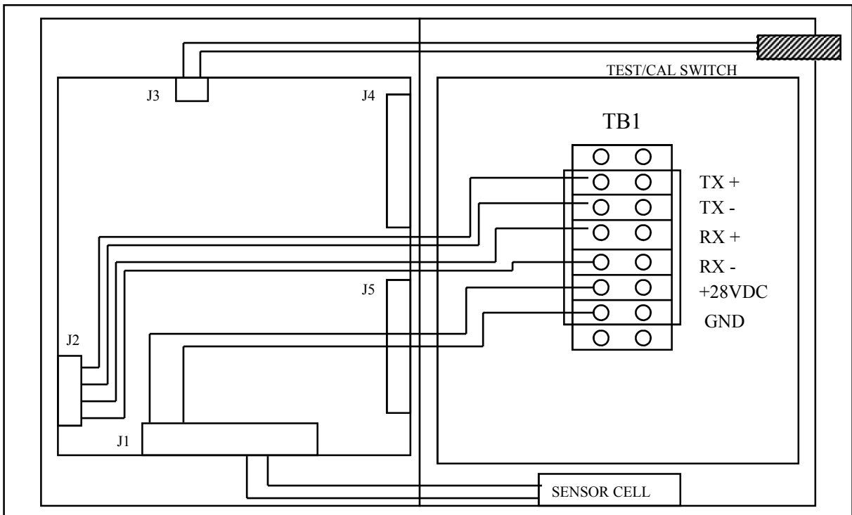
FIGURE 6, MC-4210 (4 WIRE ADDRESSABLE SENSOR)
