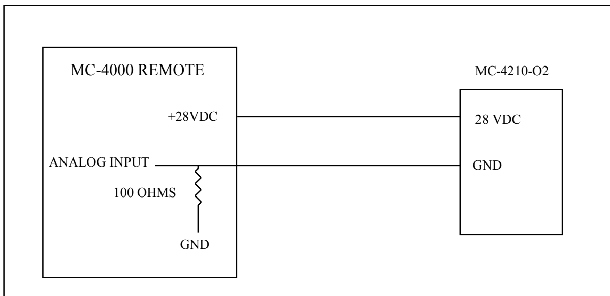
FIGURE 4, STAND ALONE CURRENT LOOP MODE CONNECTION TO MC-4000 MONITOR SYSTEM
