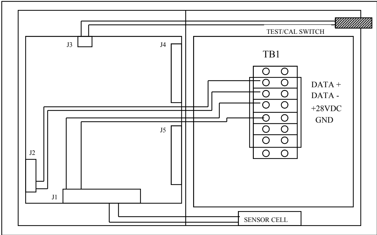
FIGURE 5, MC-4210 (2 WIRE ADDRESSABLE SENSOR)
