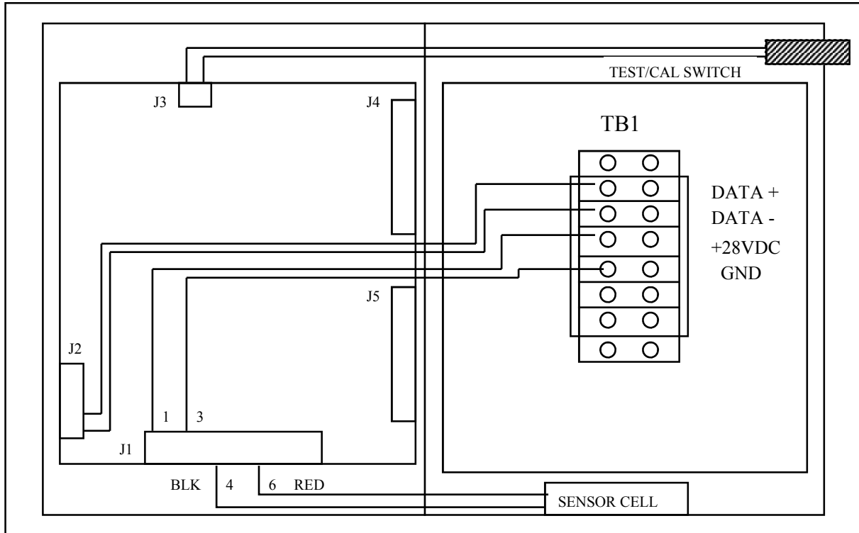
FIGURE 2, MC-4210-O2 MONITOR CONNECTIONS
